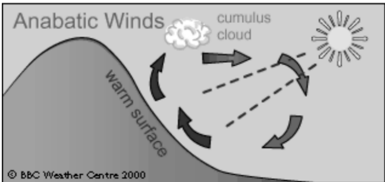
Figure 2 Anabatic Wind
